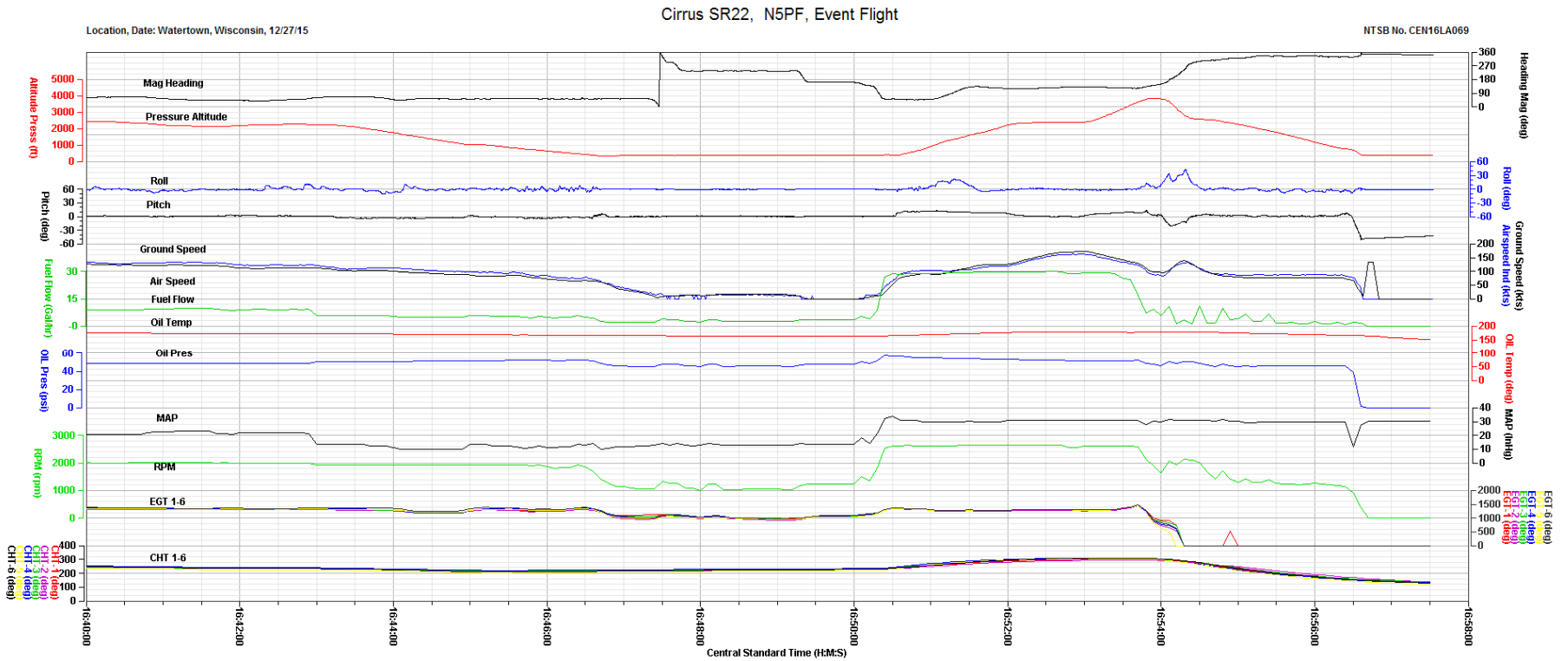
Figure 2. Plot of MFD and PFD data during last 17 minutes of event flight.
