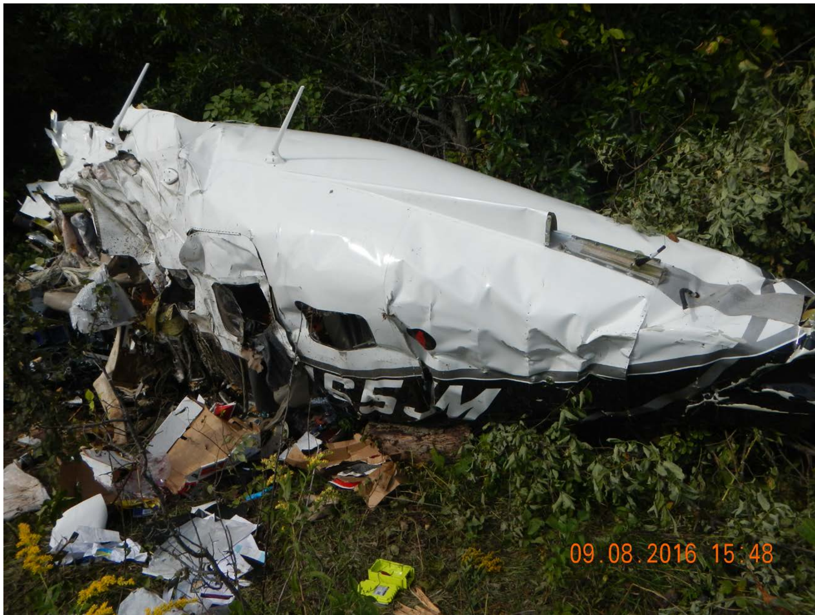
Photo 2 – Accident Site Main Wreckage Closeup
