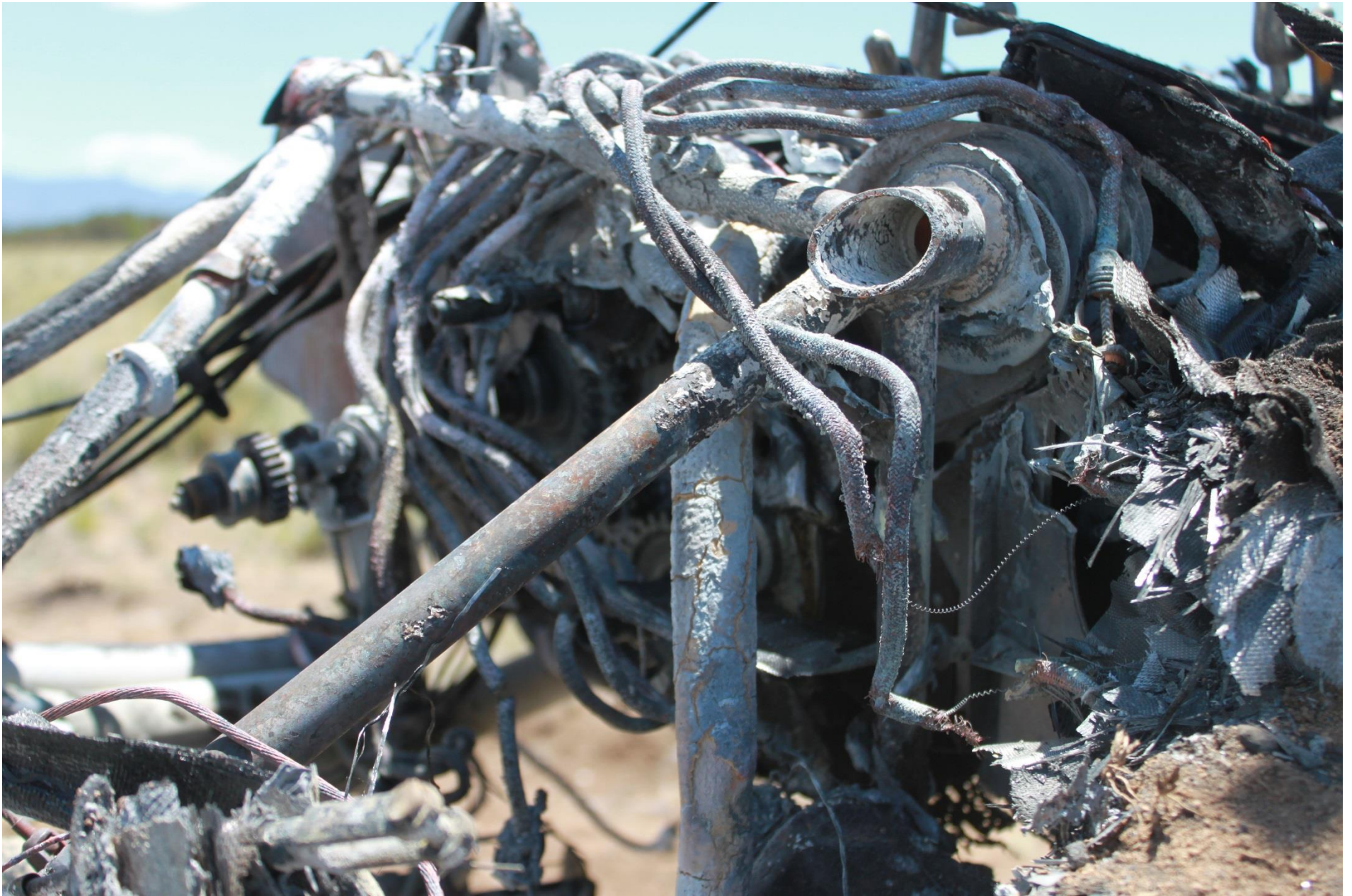
Photo 6 – View of engine accessory section
