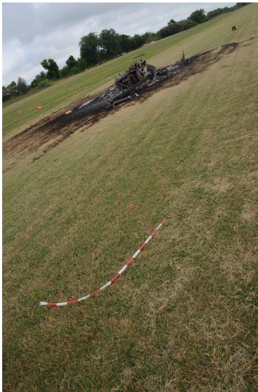
Photo 11 - View of the main wreckage and tail rotor guard.
