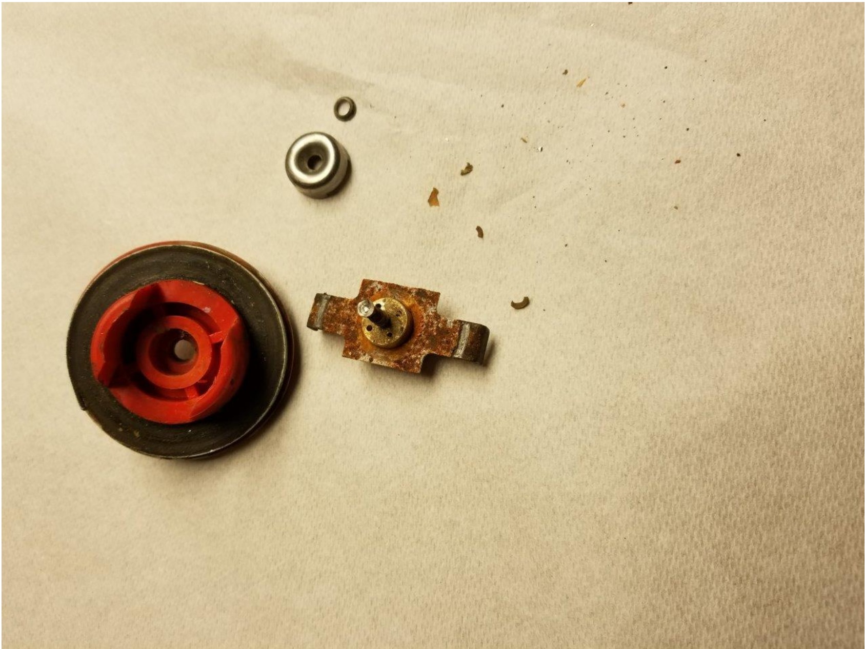
Photo 11 - View of the disassembled fuel cap.
