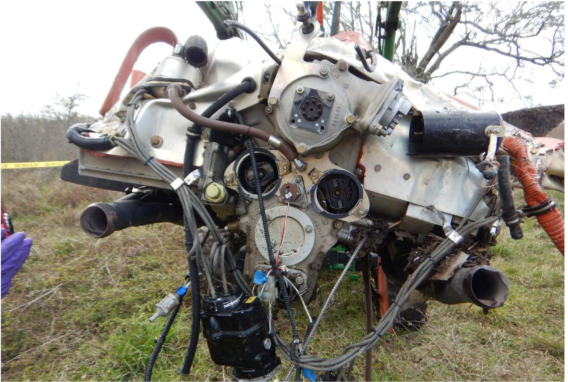
Photo 15 – Accessory Section of Engine
