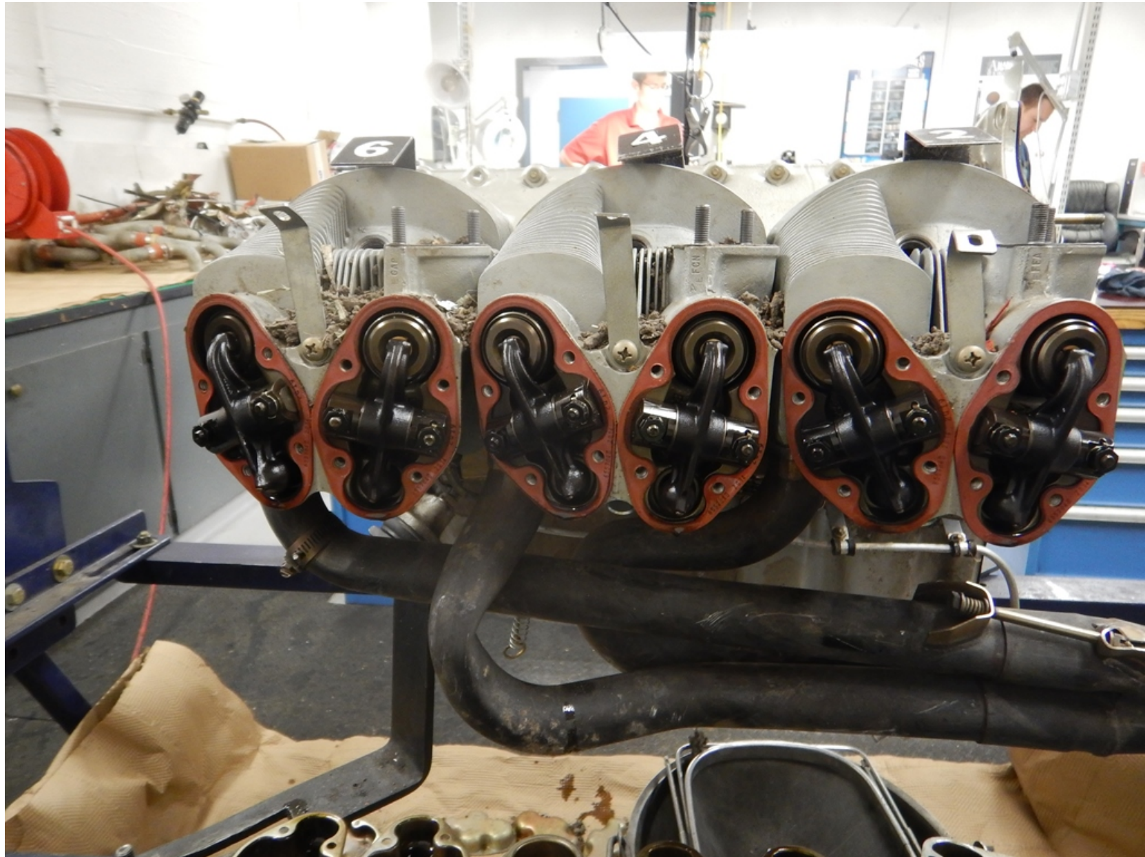
Photo 17 – Cylinders 2, 4, and 6
