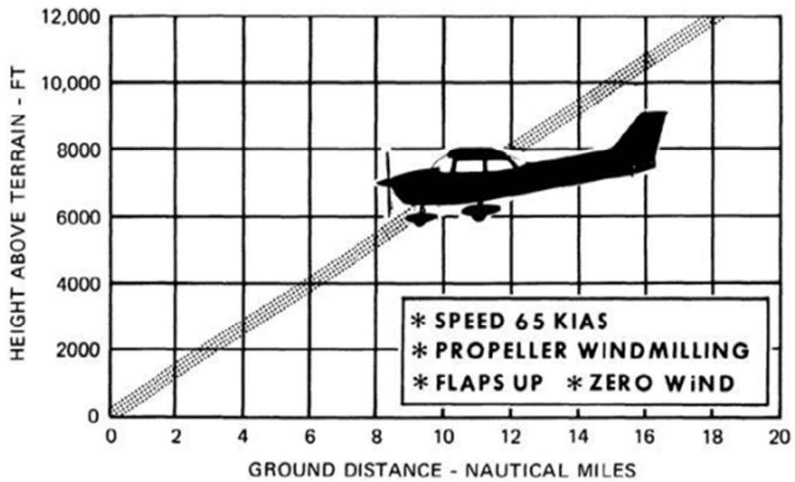
Figure 2: The Cessna 172N flight manual chart for maximum glide distance shows an approximate glide distance of 1 nautical mile at an altitude of 500 ft above ground level with a speed of 65 knots indicated airspeed, propeller windmilling, flaps up, and zero wind.
