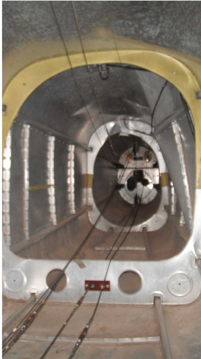
Photo 8 – Control Cables
