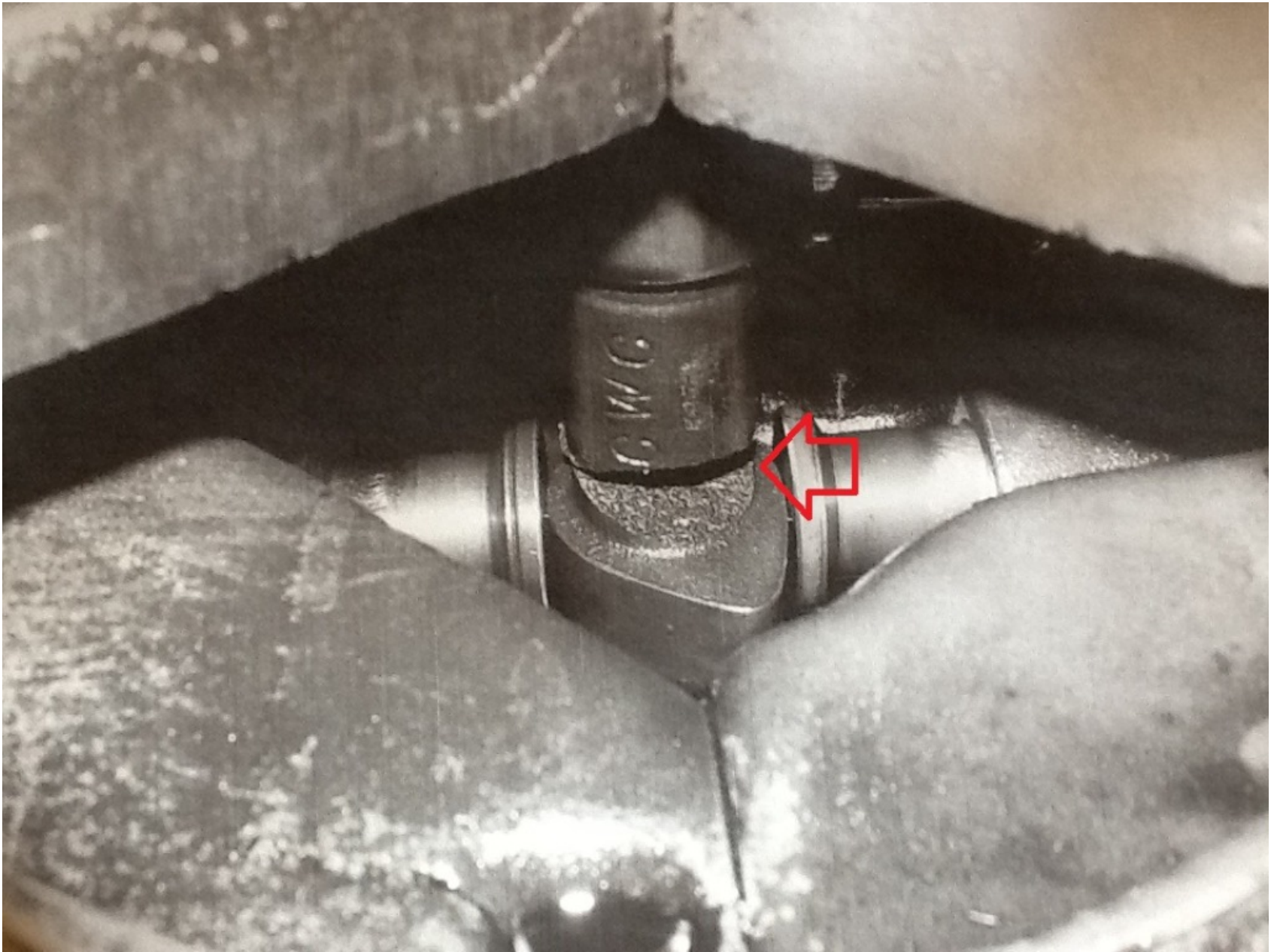
Photo 1 – Broken camshaft (non NTSB photo)
