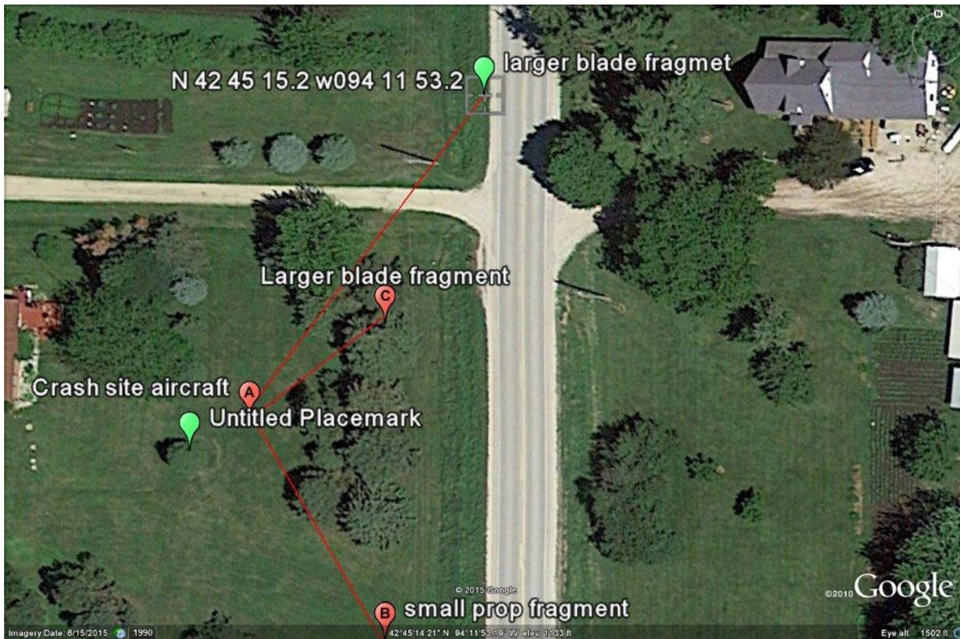
Photo 1 – overhead view of the accident site with propeller blade fragments marked
