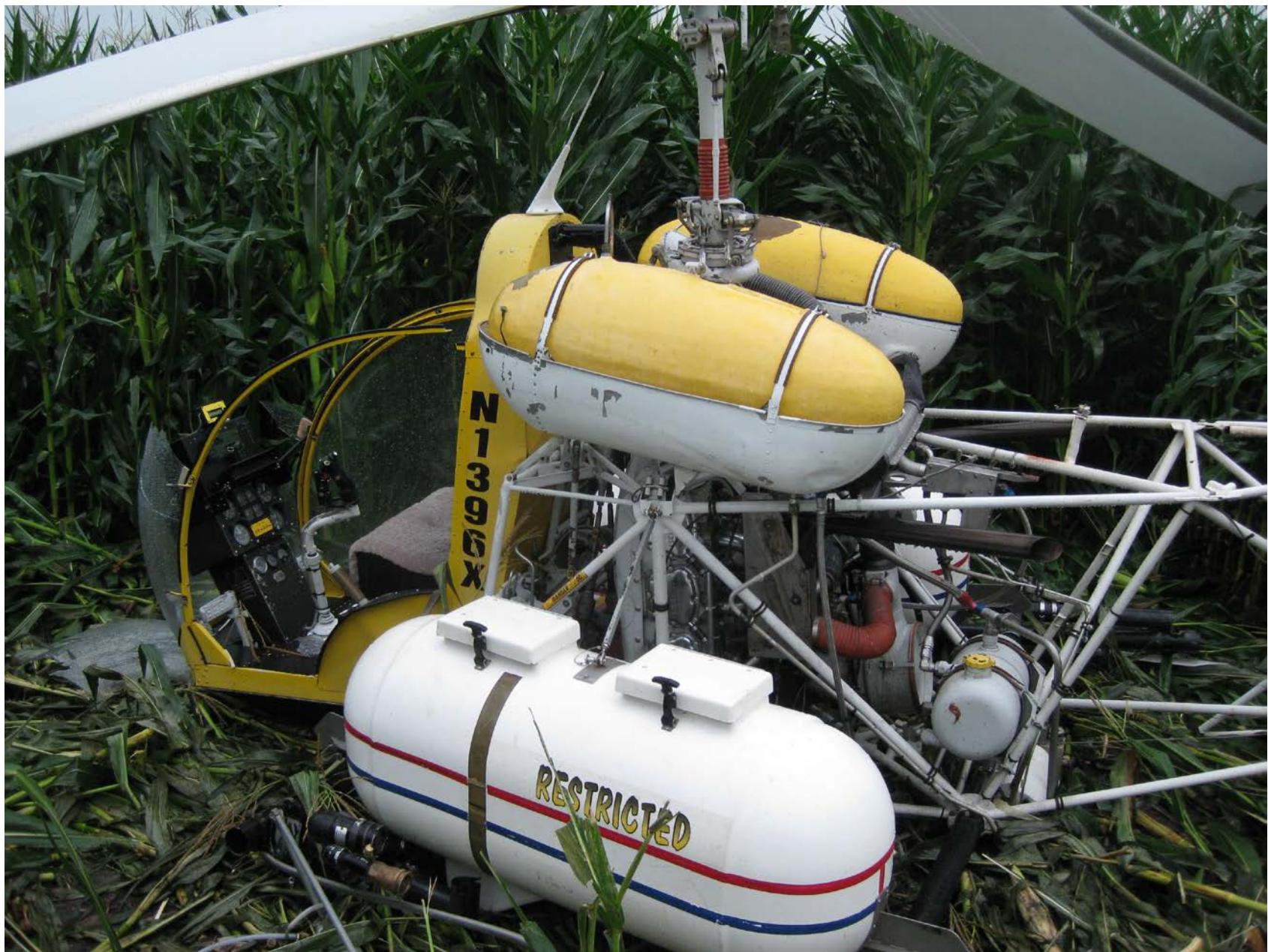
Photo 3 – Main Wreckage
