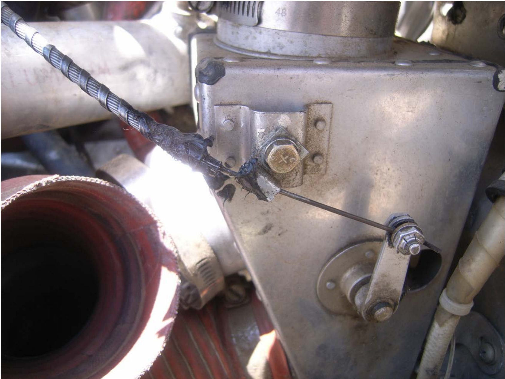
Photo 2 – The separated carburetor heat sheath and clamp.
