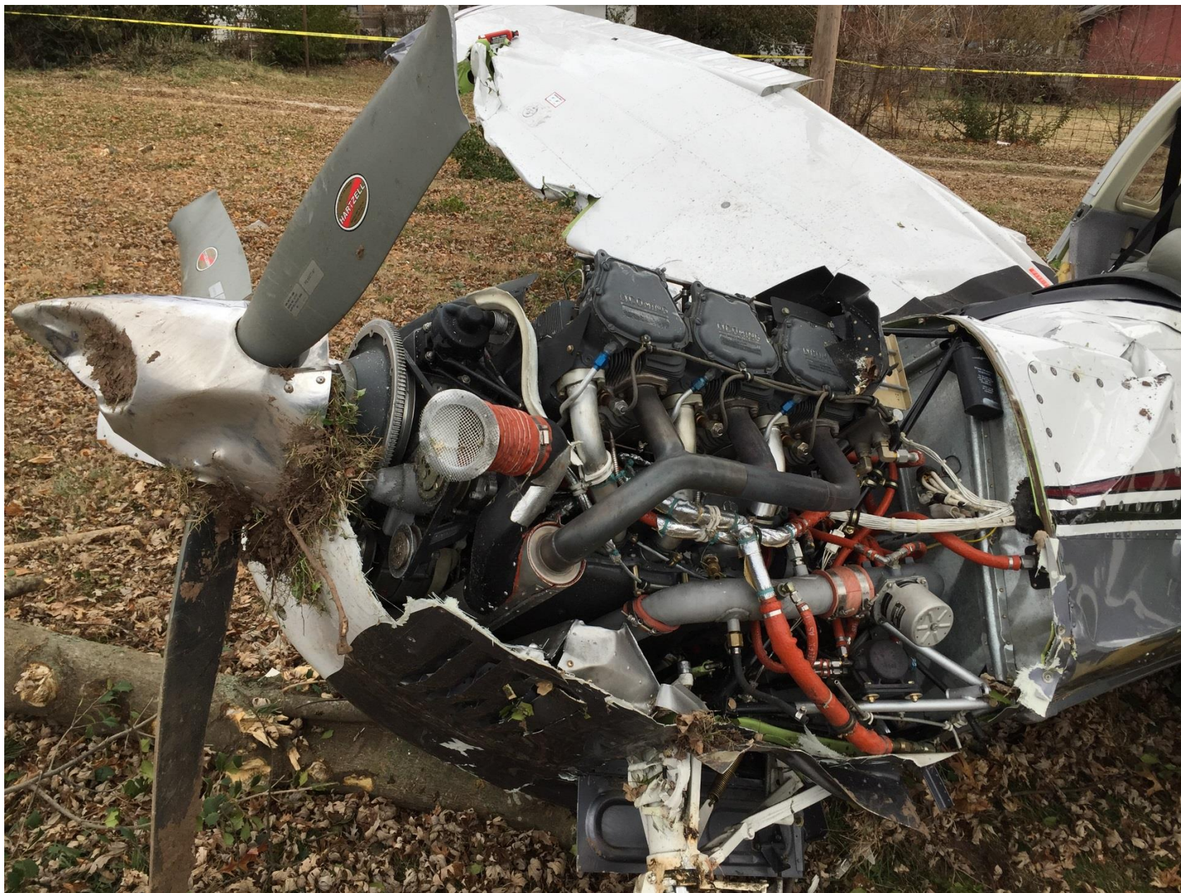
Photo 9 – Damage to the propeller and the airplane's front section. (FAA Photo)
