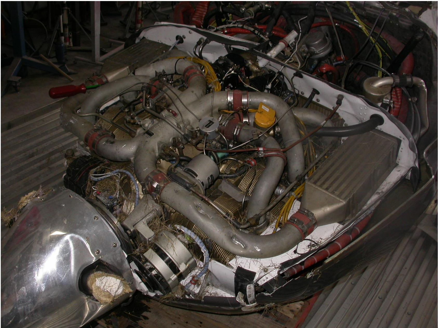
Photo 16 – View of the engine with the top cowling removed
