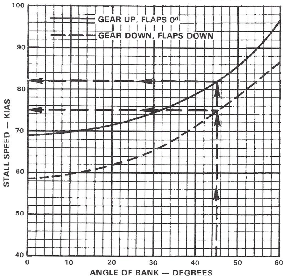
ANGLE OF BANK VS. STALL SPEED
