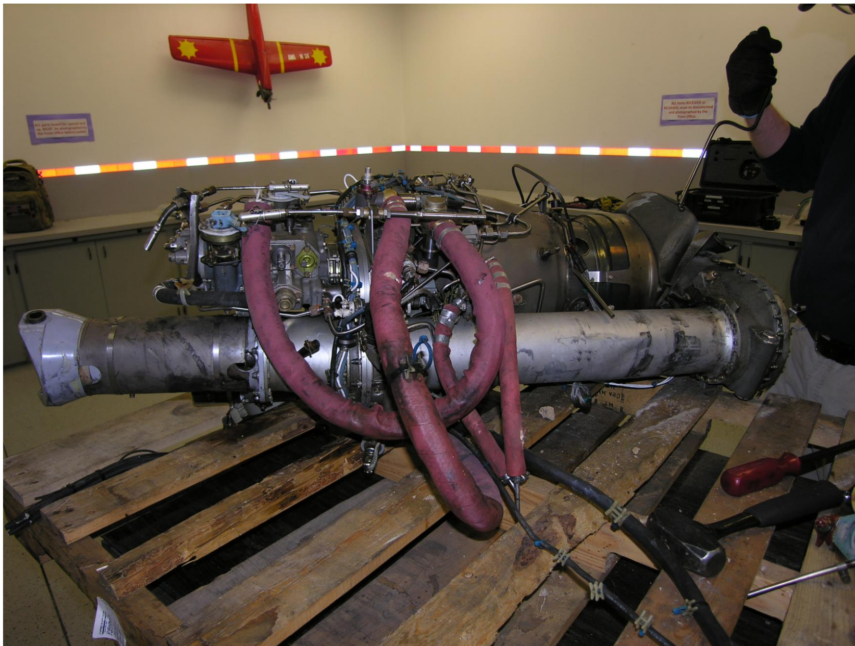
Photo 4 - Engine
