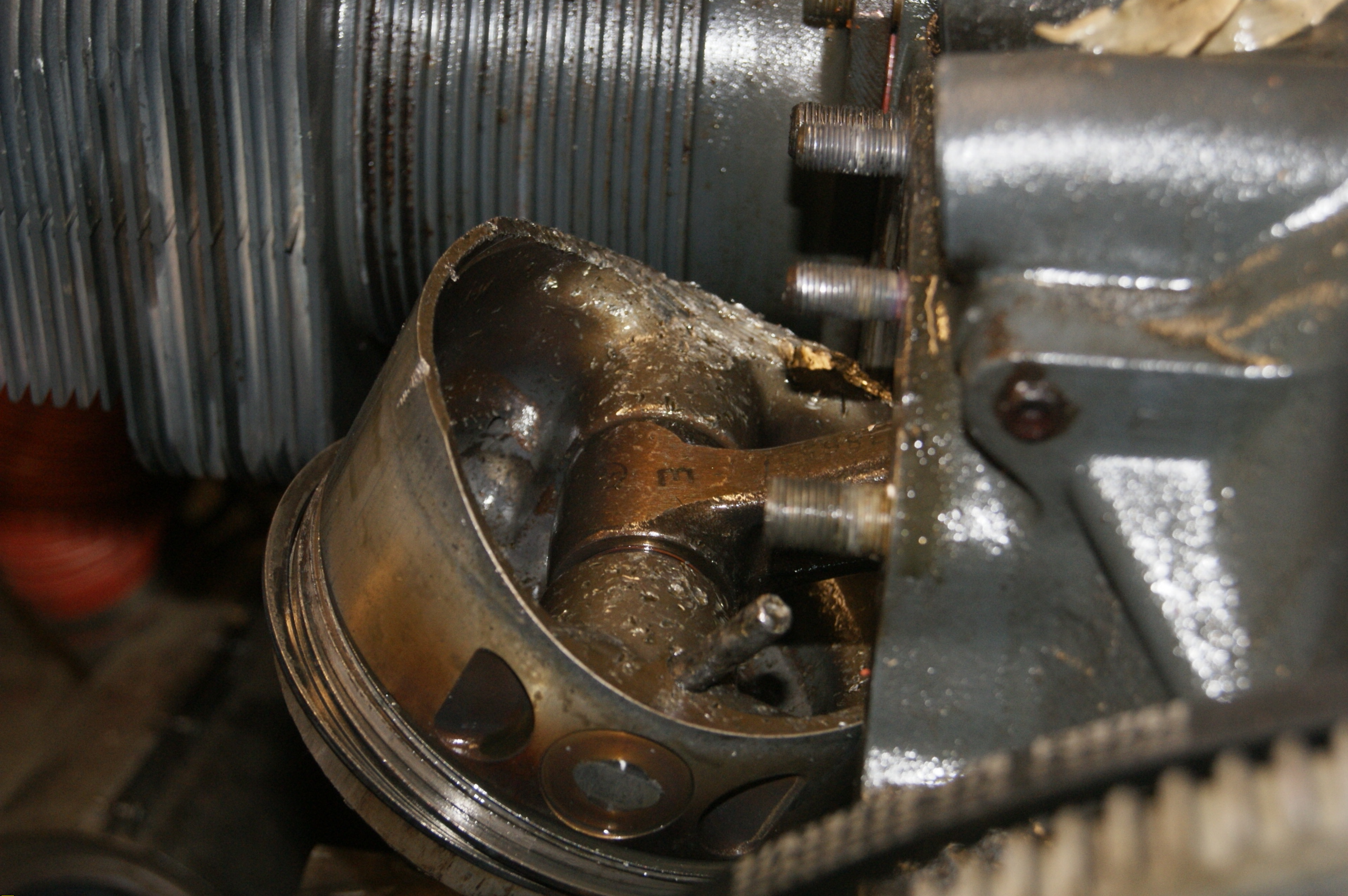
Photo 9 - Number 1 piston. Note embedded threaded stud from number connecting rod cap
