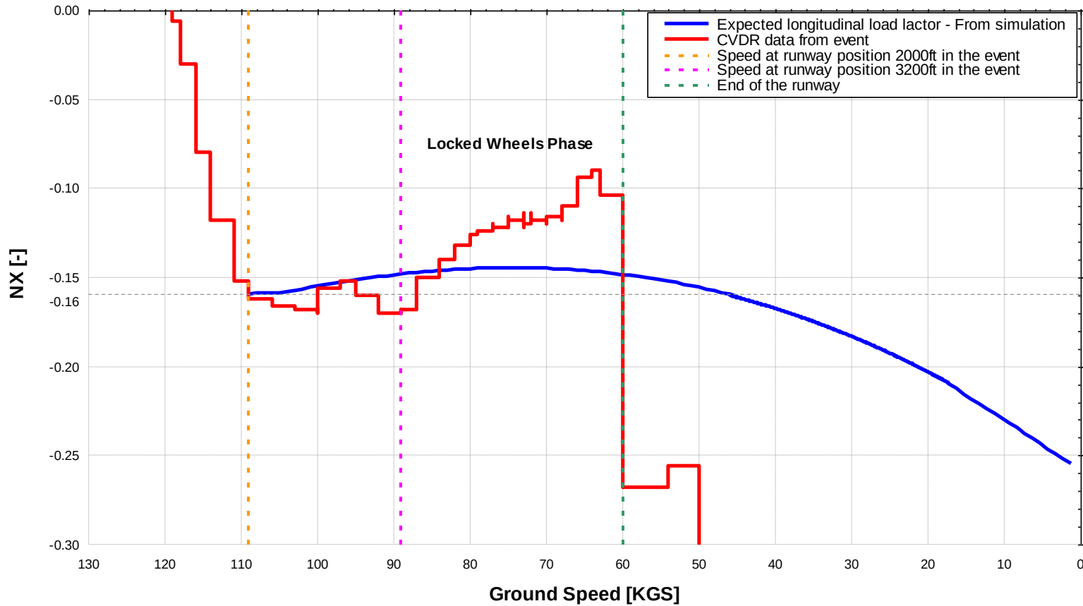
Longitudinal Load Factor vs. Ground Speed for Landing with 3mm of Standing Water
