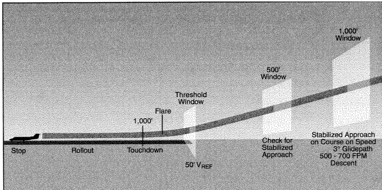
FIGURE 1-1. STABILIZED APPROACH
