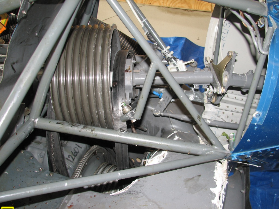
Photo 16. Upper sheave and V-belts.
