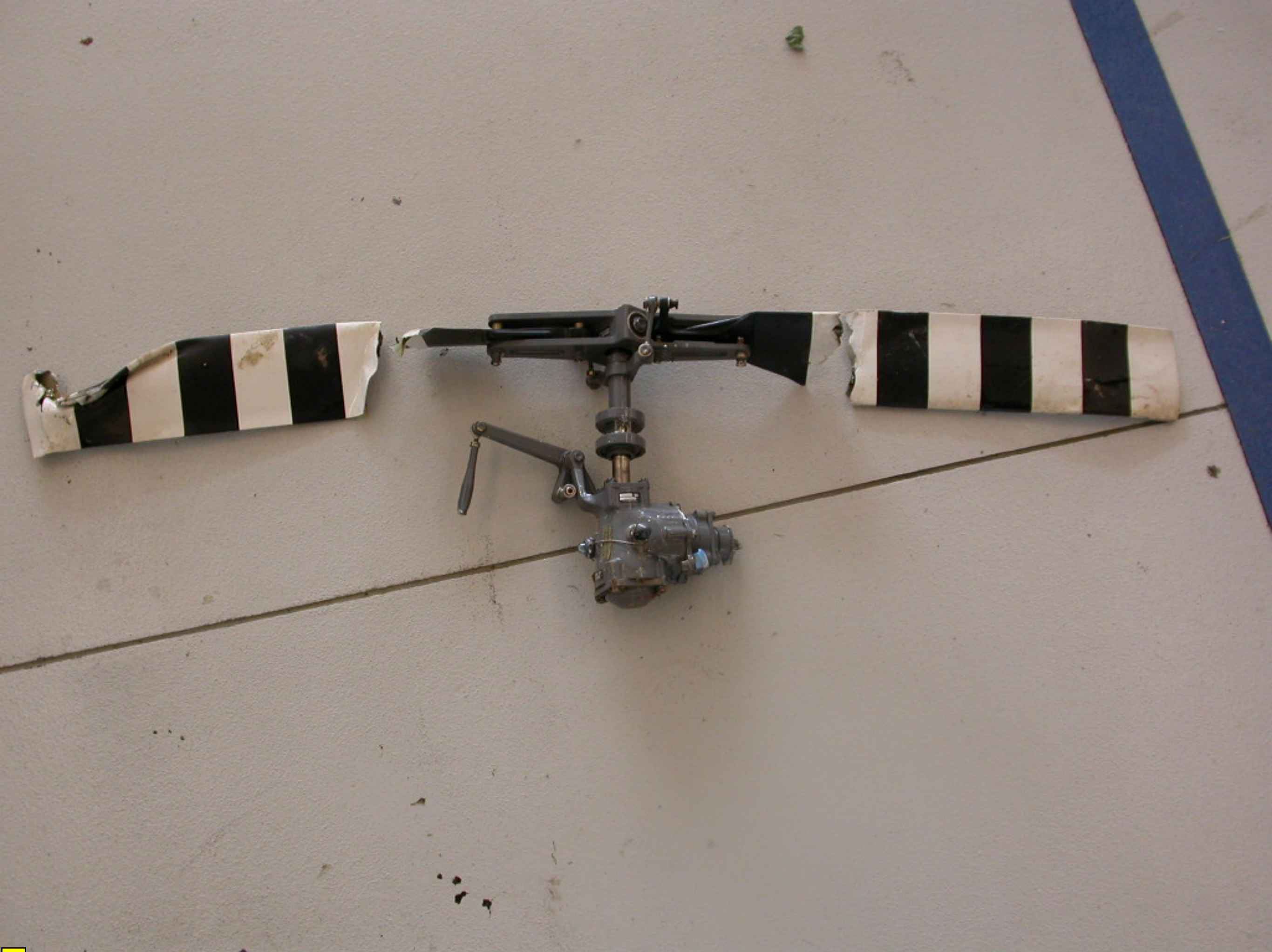
Photo 12. View of tail rotor layout.
