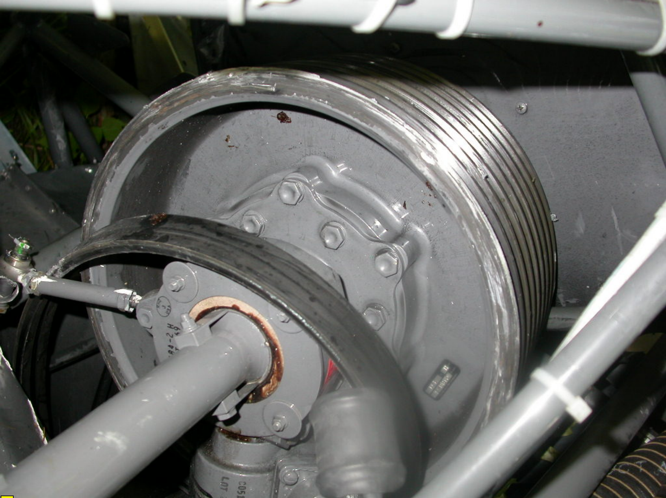
Photo 10. View of transmission drive belts and clutch.
