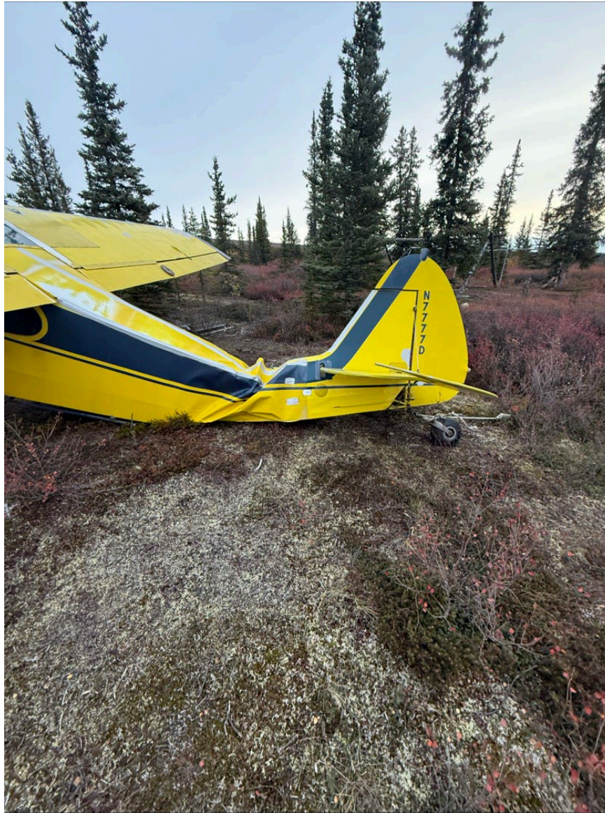
Photograph 2 - Image of fuselage and empennage (Courtesy of Owner)
