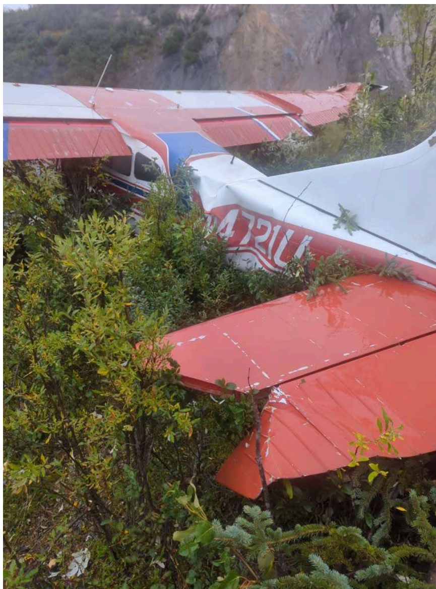
Photograph 1 - Image of horizontal stabilizer, wings, and fuselage (Courtesy of Owner)
