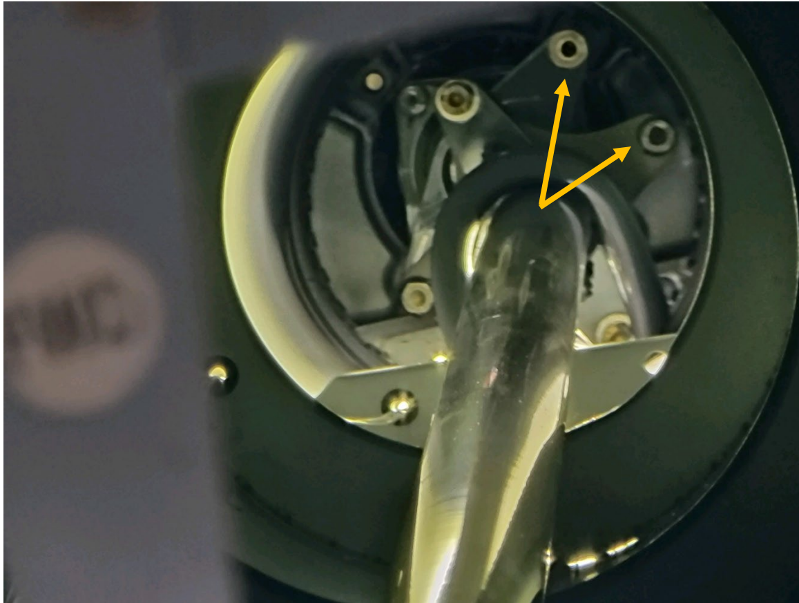
Photograph 2 - Bolt missing from flex plate yoke assembly (Courtesy of FAA)
