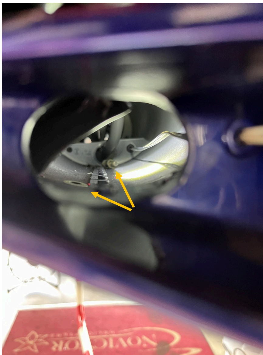
Photograph 3 - Bolt and washer from flex plate assembly in tail boom (Courtesy of FAA)
