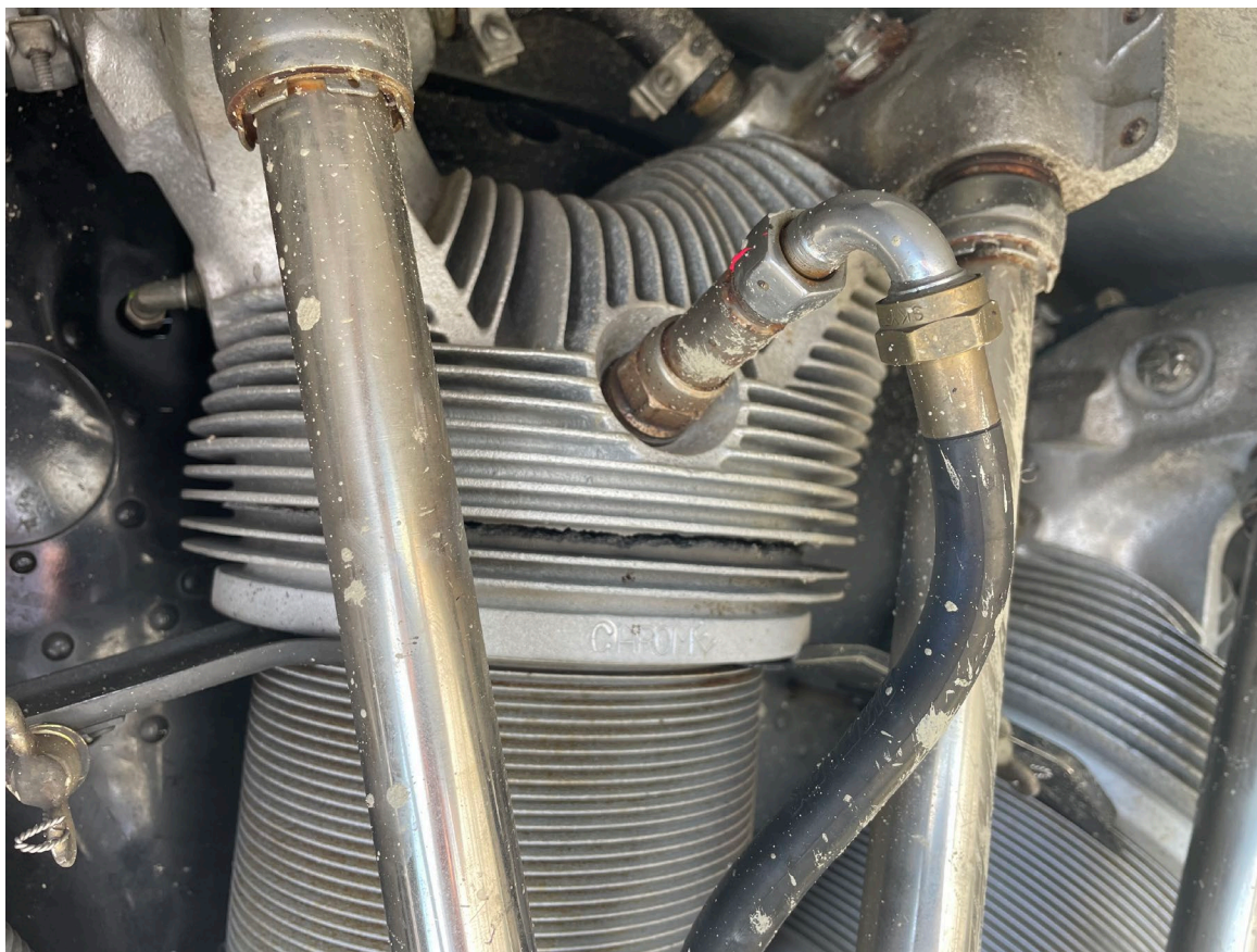
Photograph 3 - View of the cracked No. 9 cylinder (Courtesy of FAA)
