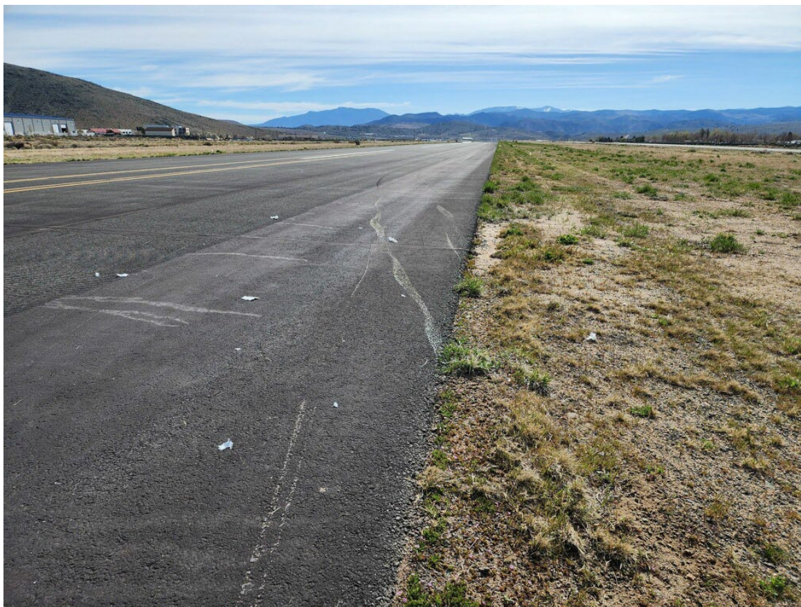
Photograph 3 - View of impact marks on runway (Courtesy of Owner)
