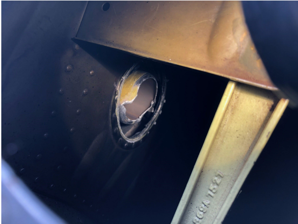
Photograph 5 - View of the damage to the tail rotor drive shaft (Courtesy of FAA)
