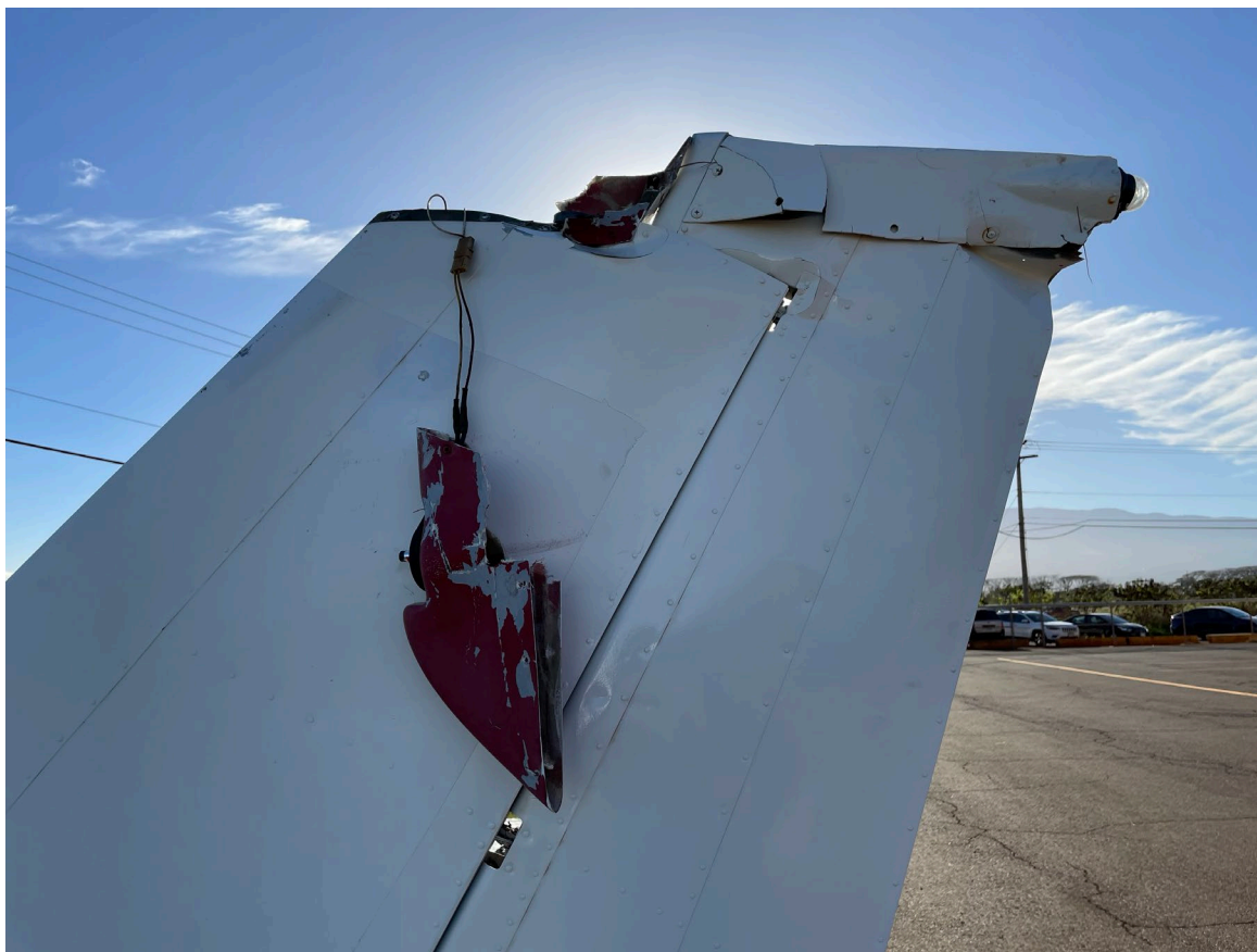
Photograph 1 - Image of the vertical stabilizer and rudder (Courtesy of FAA)
