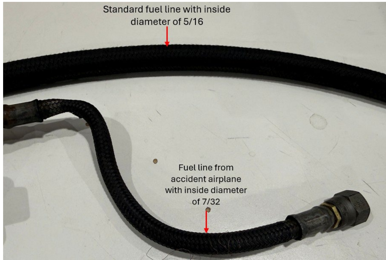
Photograph 4 View of a standard fuel hose (above) and the steel braided hose installed on the airplane (below).
