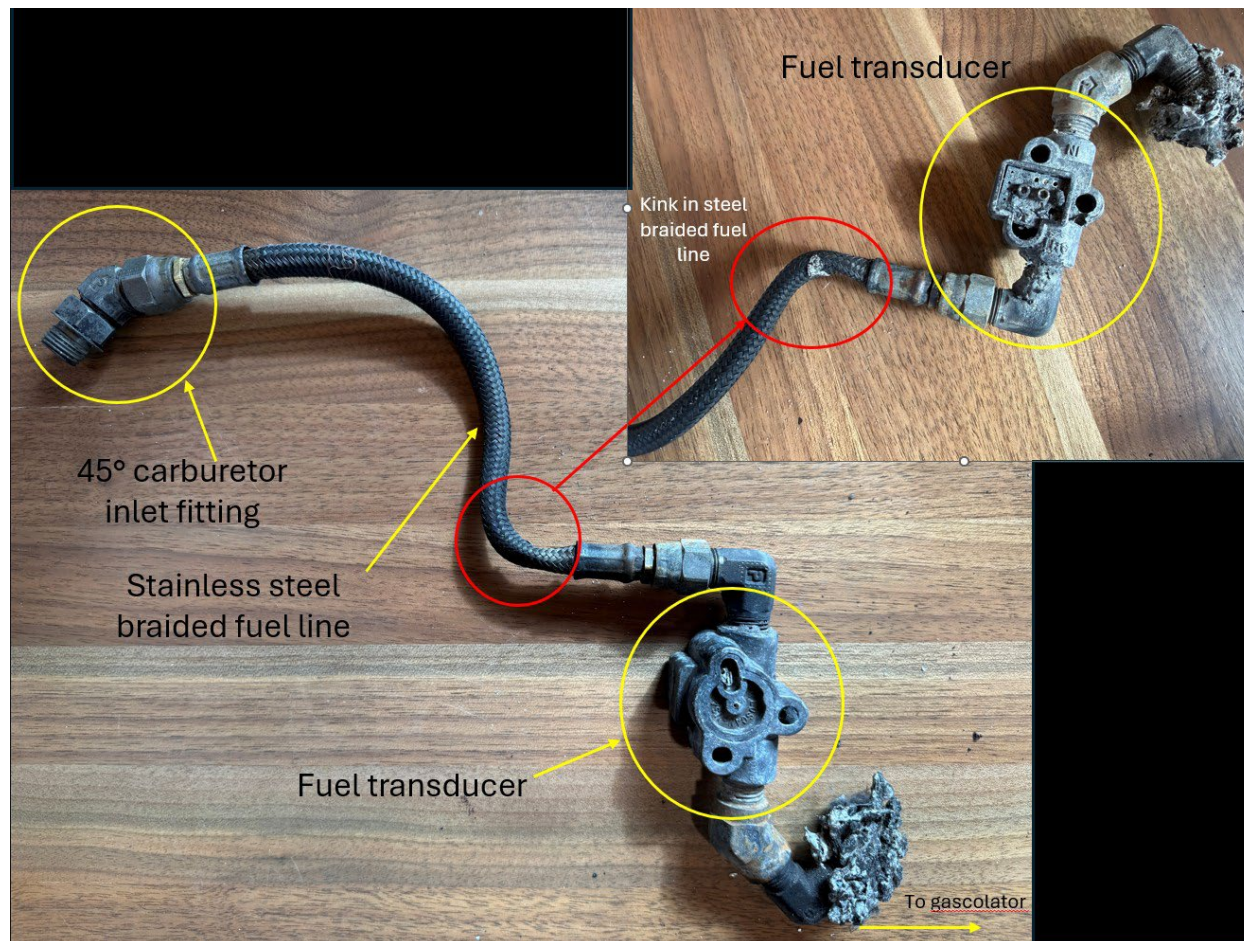
Photograph 5 View of the kink in the steel braided hose from the carburetor to the gasoclator.
