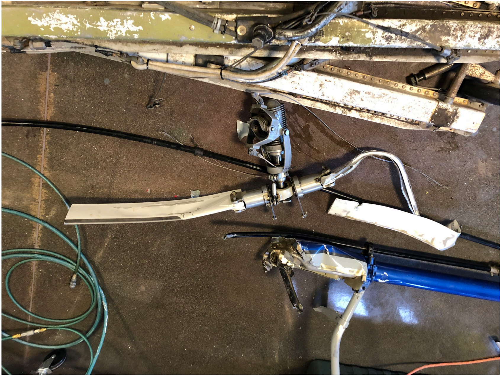
Photo 4 – View of accident helicopter’s tail rotor assembly. Photo provided by NTSB.
