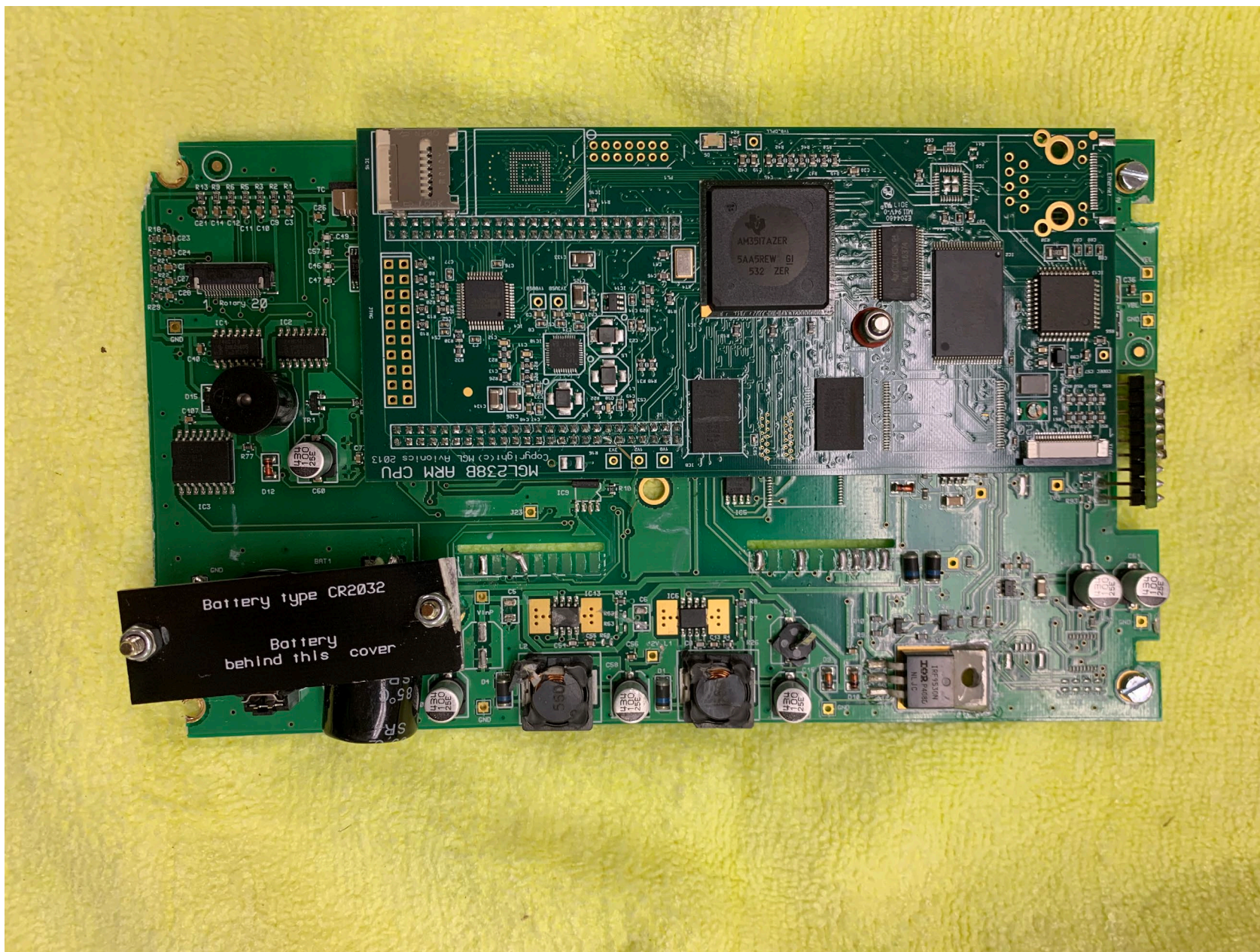
Photo 5 – Side B of Circuit board from MGL Avionics iEFIS Discovery Lite.
