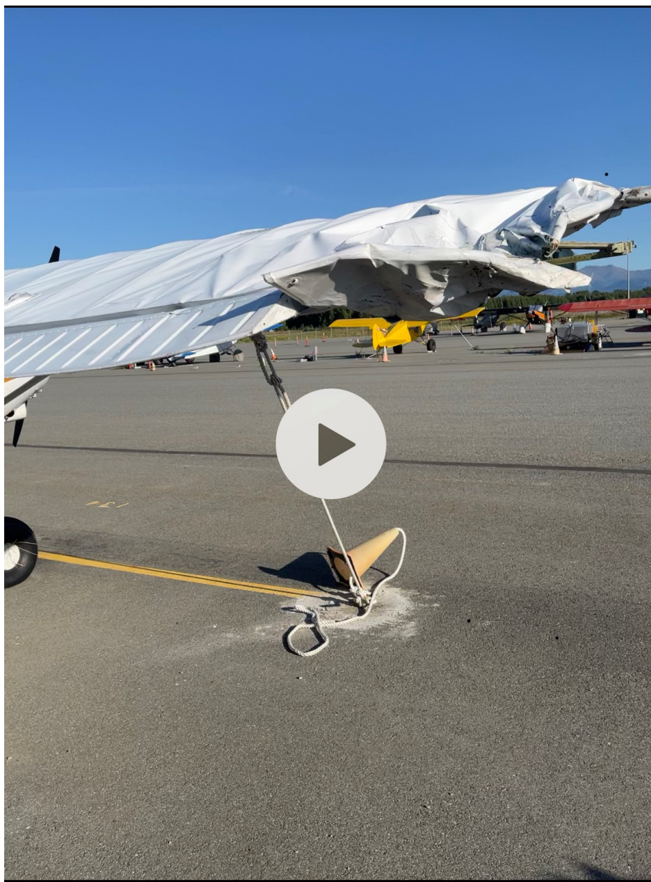
Photo 1 – Accident airplane's damaged right wing. Photo provided by the pilot.
