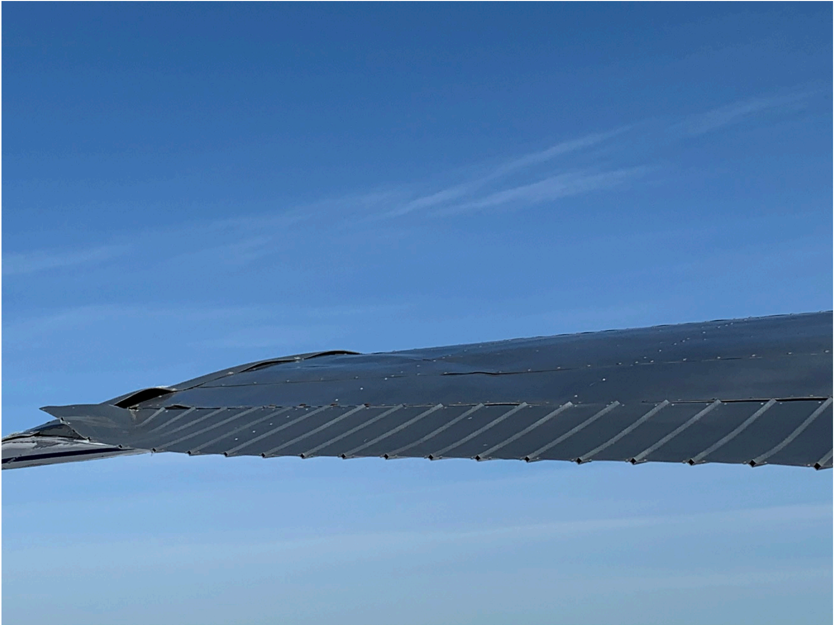
Photo 2 – Accident airplane's damaged left wing and aileron.
