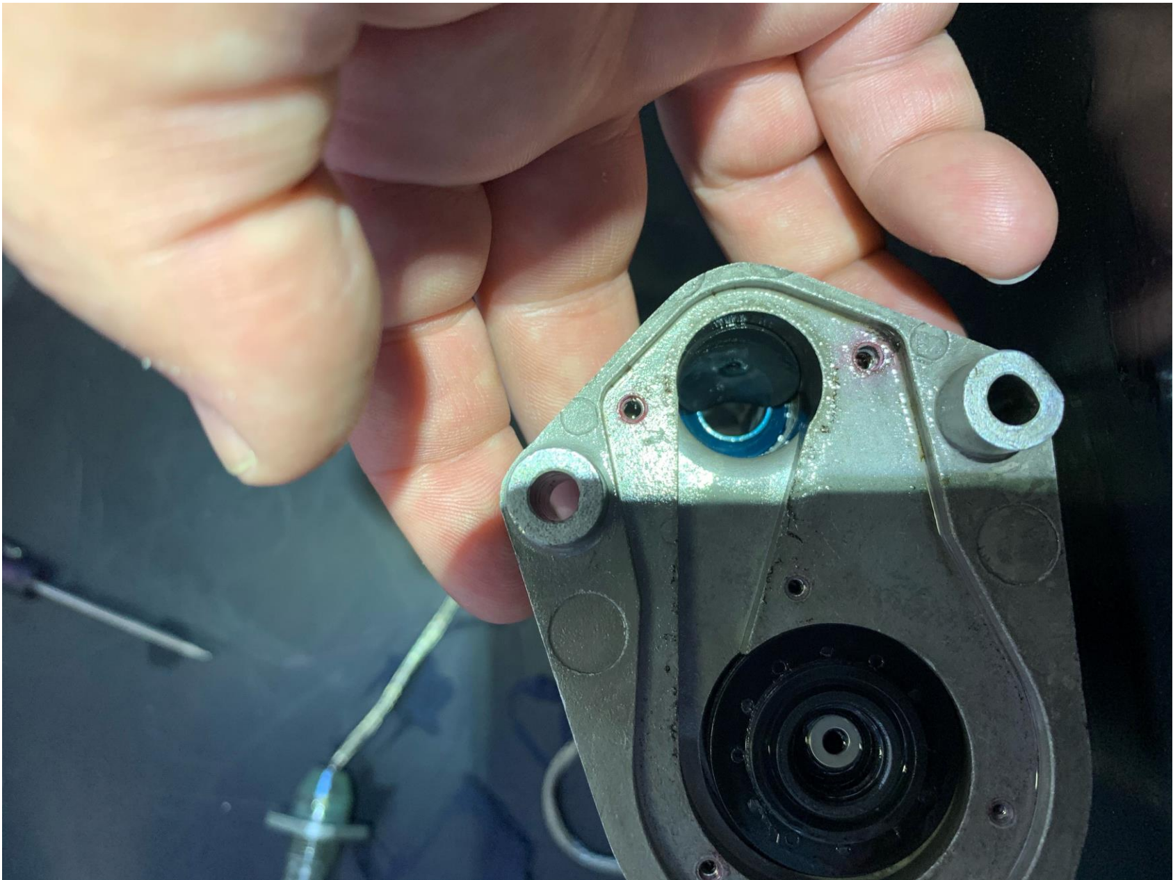
Photo 3 – Internal view of the accident fuel pump (Photo courtesy of the FAA)
