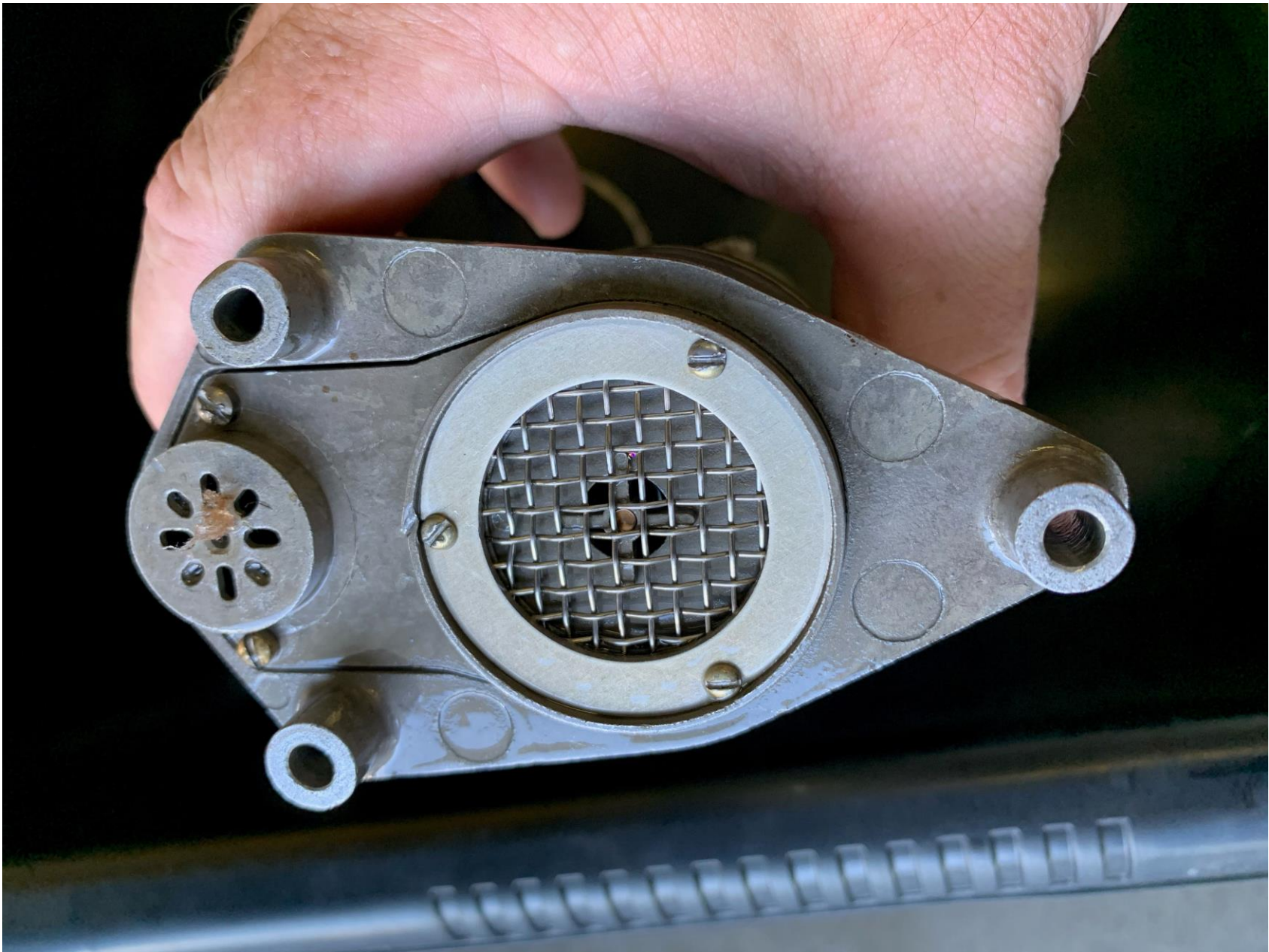
Photo 1 – View of the accident fuel pump (Photo courtesy of the FAA)
