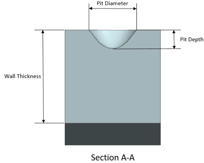
Figure 4: Corrosion Pit Geometry
