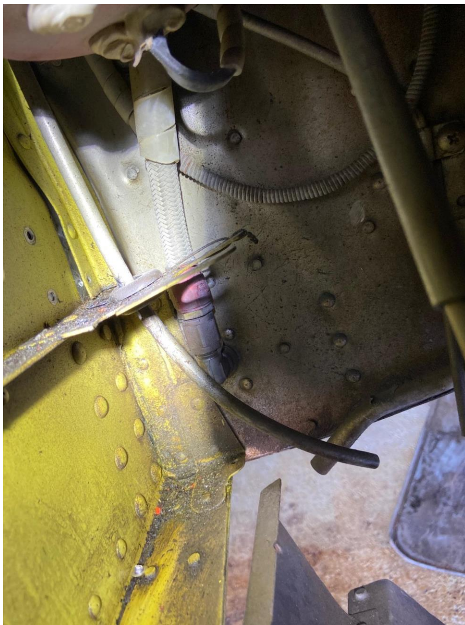
Photo 3 – View of damaged engine mount (Photo courtesy of the FAA)
