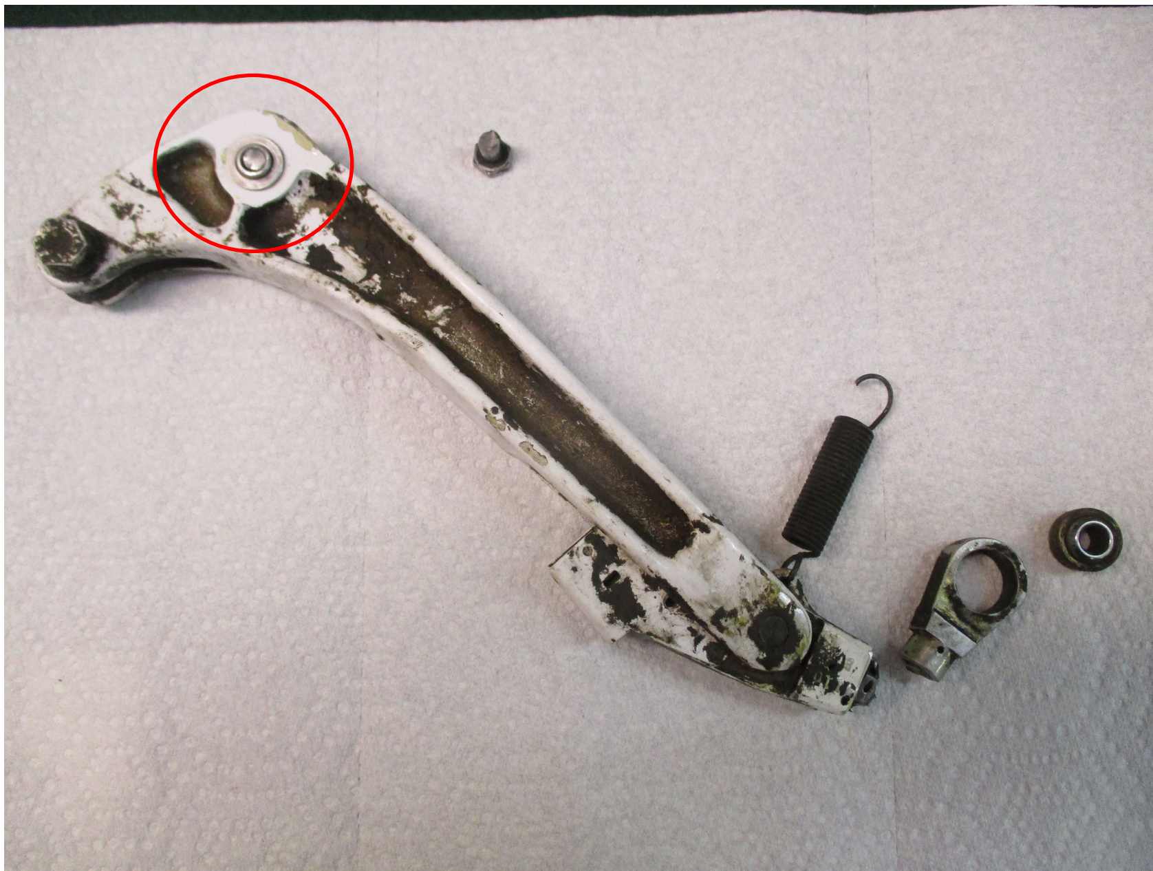
Photo 1 – Accident airplane's right main landing gear bellcrank assembly. Sheared bellcrank pivot bolt outlined in red circle.
