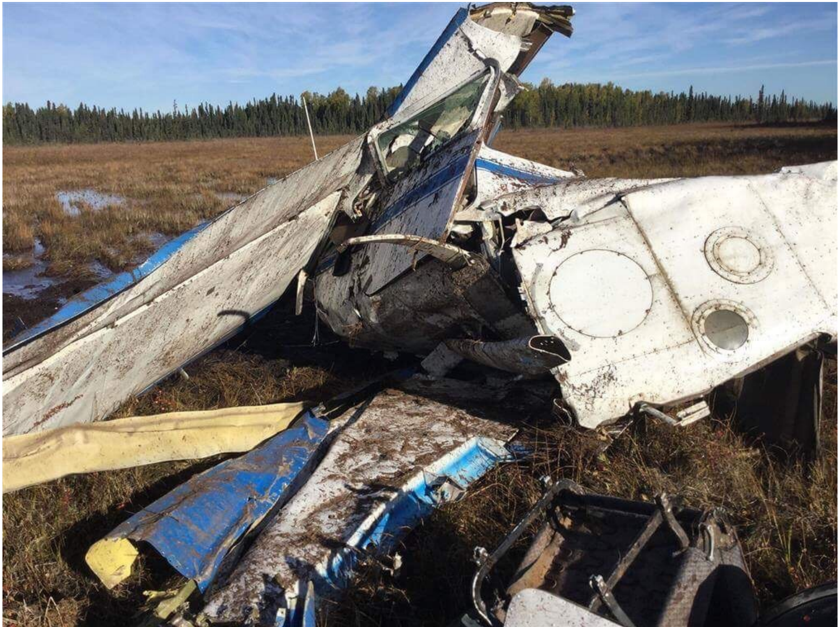
Photo 3 - Rear view of N8070Z wreckage (courtesy of airplane owner)
