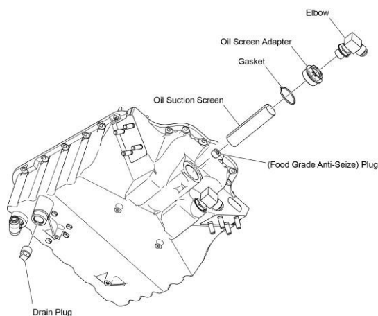
Figure 4 Example of an Oil Drain Plug and Oil Suction Screen on AEIO (Aerobatic Engines)
