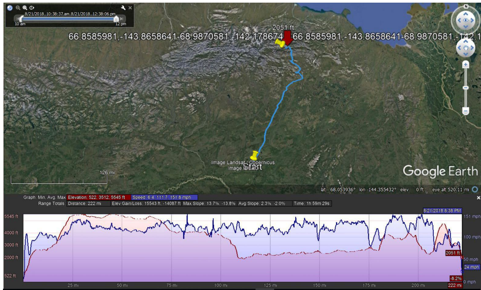
Figure 2. Leg 2 GPS track data and elevation profile.
