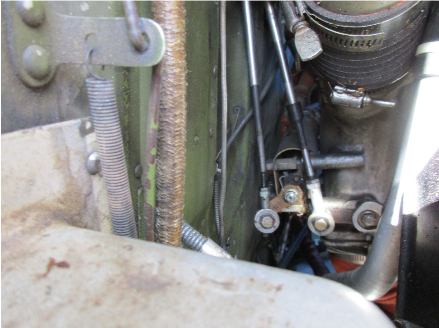
Photo 5 - Engine control linkages. (Source: FAA)
