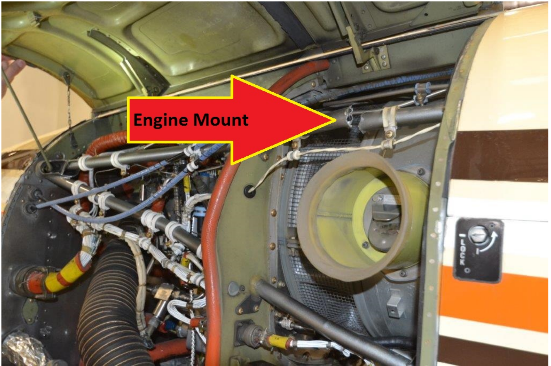
Photo 6 – View of the fractured right engine mount (courtesy of Bering Air).
