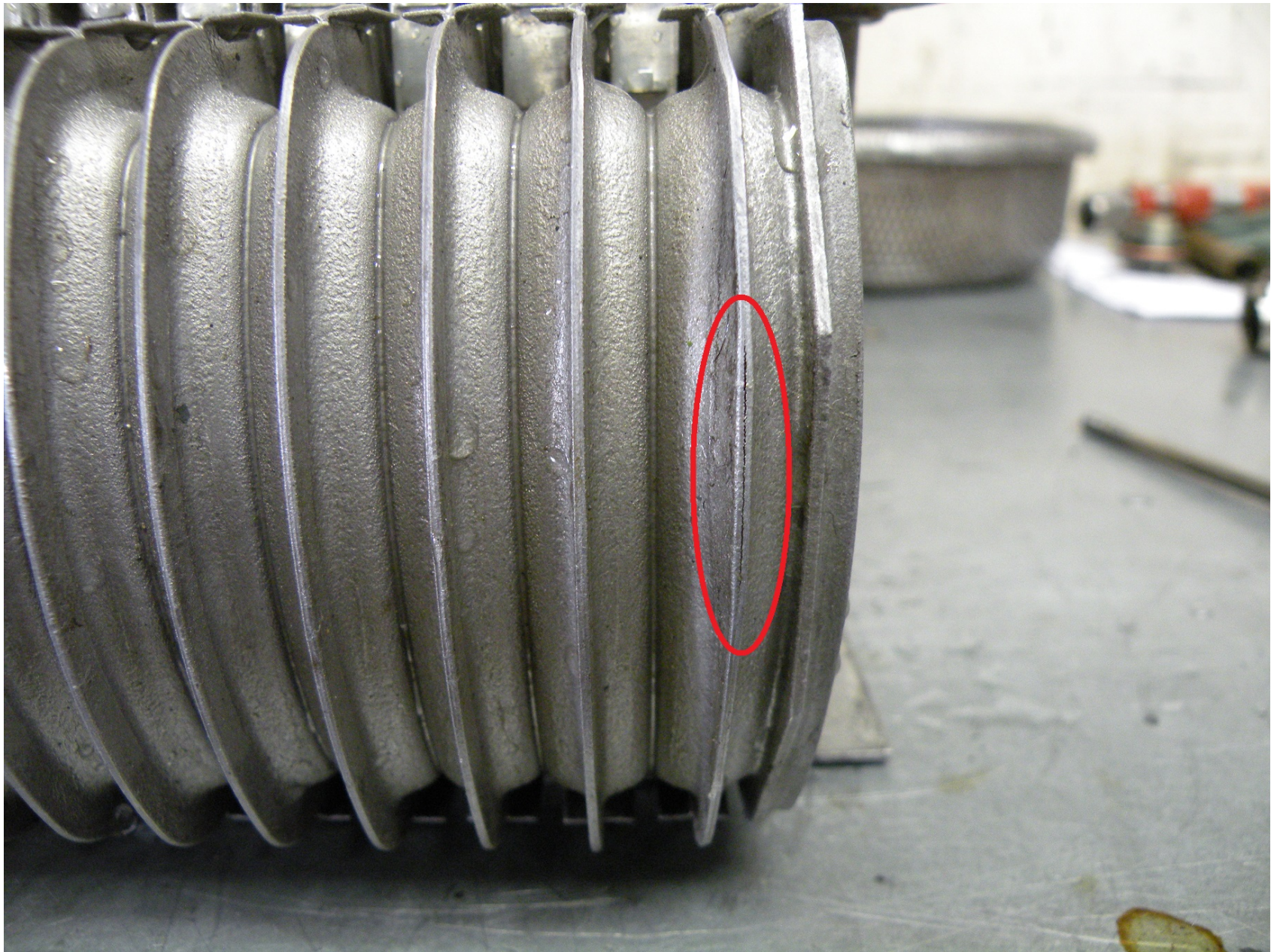
Photo 6 - Right oil cooler (Aero-Classic P/N 8000074) with fracture at the brazed plates.
