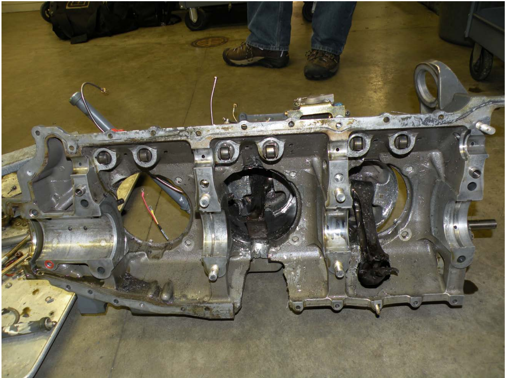
Photo 4 - No. 3 and 5 pistons and connecting rods exhibiting thermal damage and fractures.
