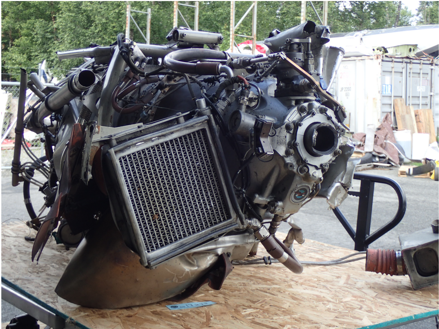
Photo 8 - Pratt & Whitney PT6-114A turbine engine indicating fractured shaft
