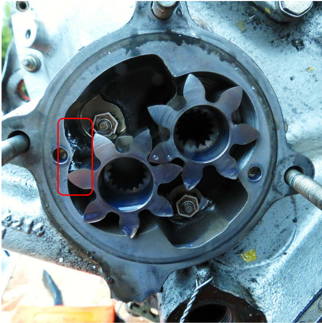
Photo 9 - No. 3 and 4 bearing scavenge pump indicating metallic debris
