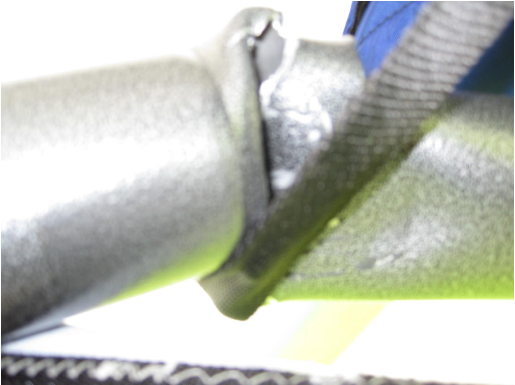
Photo 1 – View of wing keel (courtesy of the FAA)
